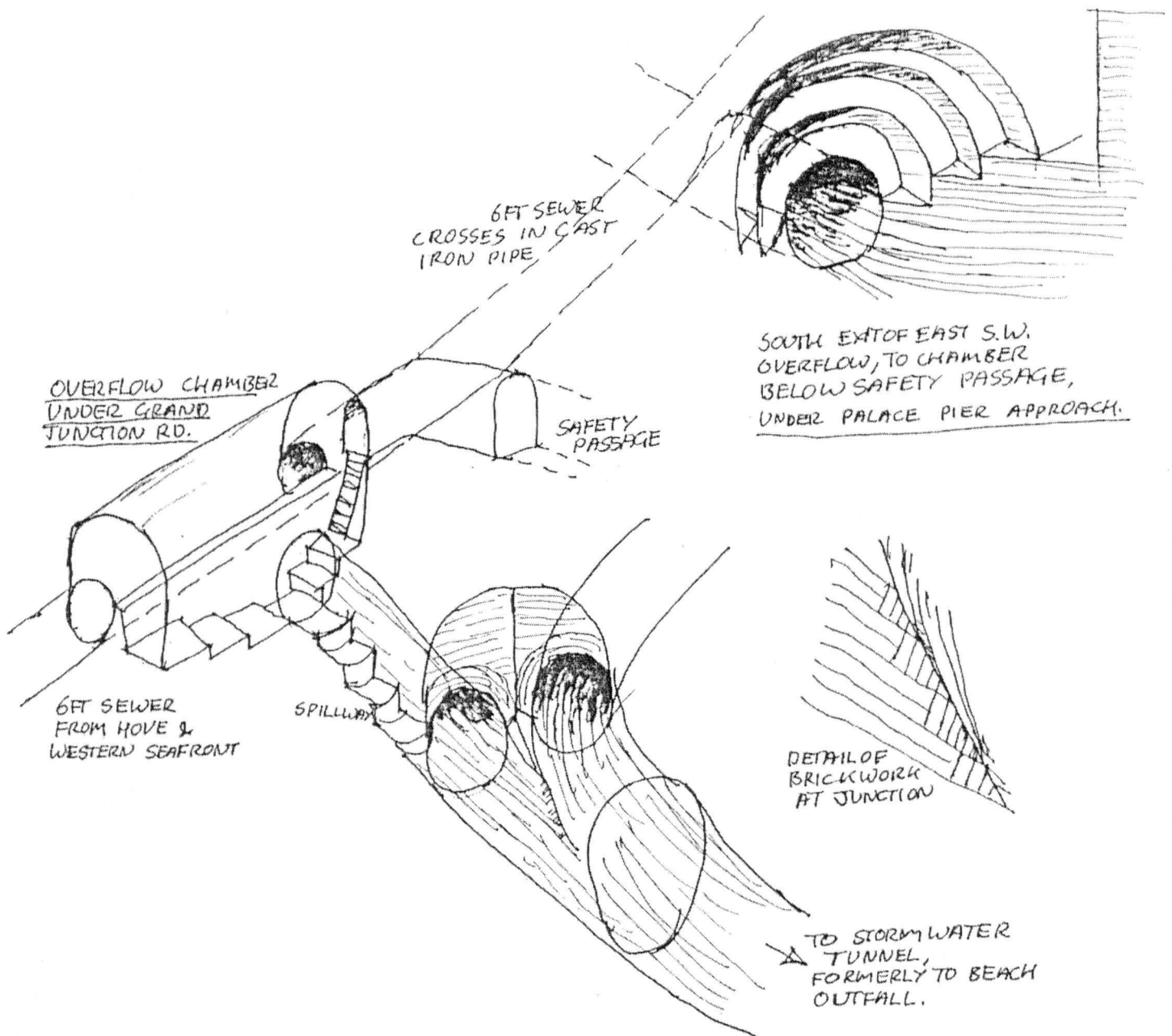
Fig. 1 Brighton Sewers
