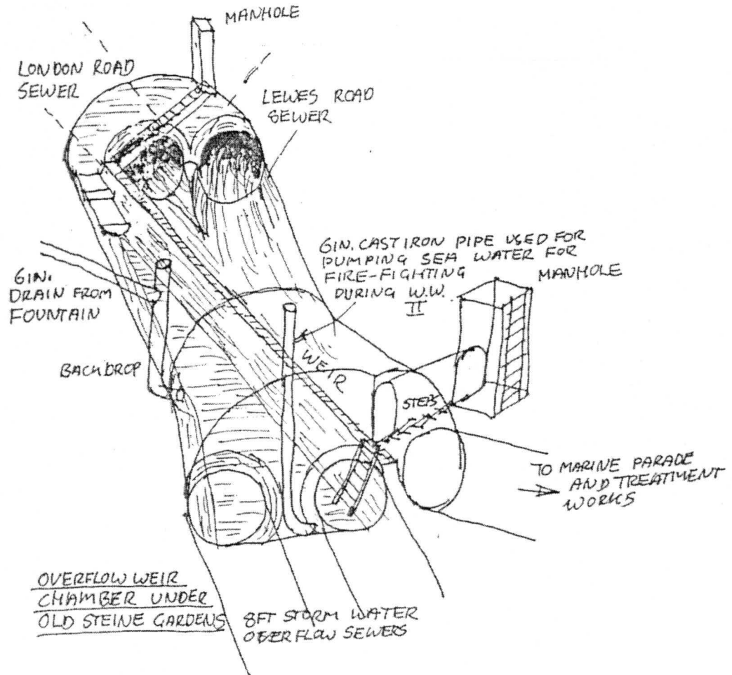
Fig. 2 Brighton Sewers; Overflow chamber under Old Steine Gardens Drawn by Martin Hammond, June 2000
